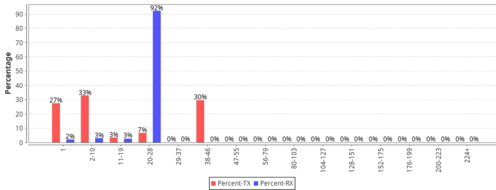
N 2.4Ghz WiFi Packet AMPDU Length Percentages
