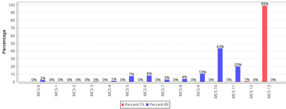
BE 5Ghz WiFi Packet MCS Percentages
